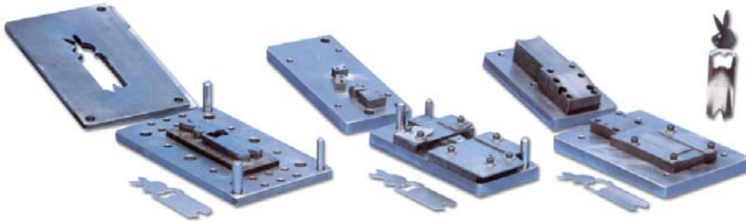
Examples of short-run, semi-permanent blank, pierce and form tooling.
